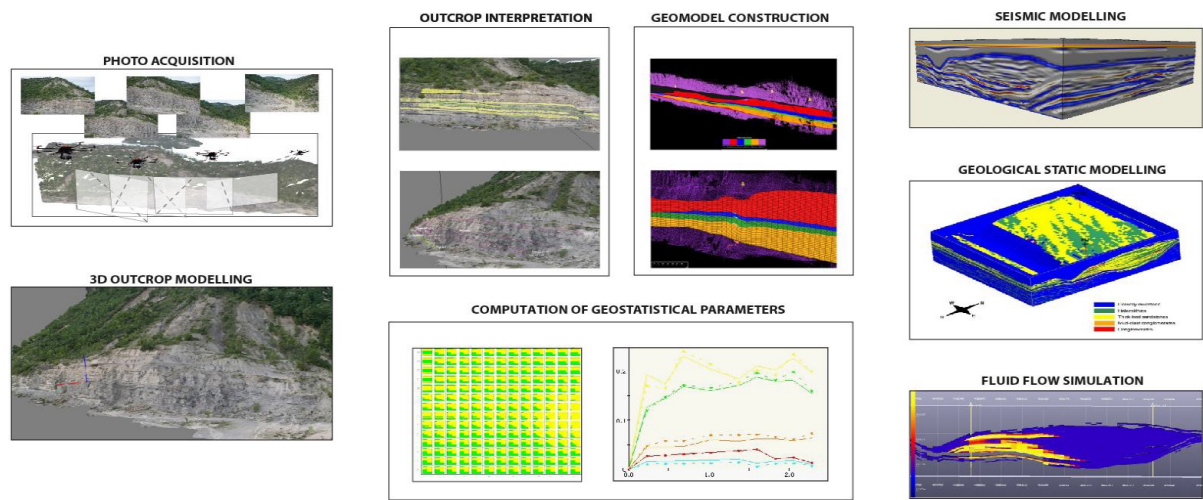
Figure 1: A turbiditic reservoir analog, Ainsí quarry, Spain
